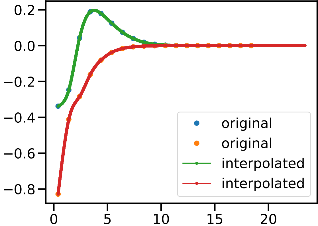
Hamiltonian Interpolation After Training (14, 14, 1, 1)
